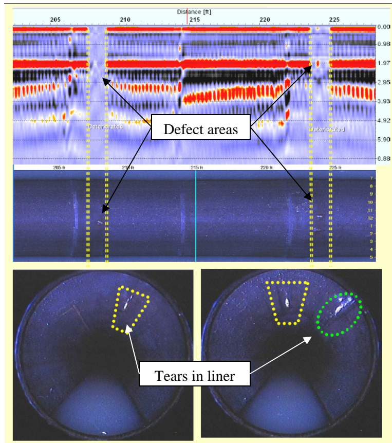
Figure 8. In-pipe ground penetrating radar results
