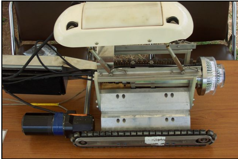
Figure 5. Prototype inspection robot with gpr unit
